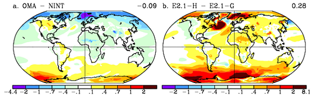
Figure 11. Differences of surface air temperature change, 2081–2100 minus 1995–2014 (°C) in different climate models for the SSP2-4.5 scenario. (a) One-Moment Aerosol–non-interactive; (b) E2.1-H–E2.1-G.
