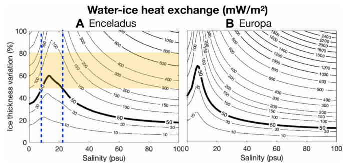
Fig. 5. The water-ice heat exchange in equatorial regions. (A) Enceladus and (B) Europa. Equation 7 is used to estimate the heat exchange rates for various salinities and equator-to-pole percentage ice thickness variations (equatorial minus polar ice thickness divided by the mean). Two-degree poleward-thinning structure is assumed and physical parameters are defined in Table 1. Parameter regimes that are consistent with observations are shaded in yellow: The ice shell of Enceladus is thought to have large thickness variations (14–18). The 50 mW/m 2 contour is highlighted by a thicker curve; heat exchange rates that exceed this are considered unphysical as the equatorial ice sheet of both Enceladus and Europa only allow ~40 mW/m 2 or so of heat flux to conduct through. Our simplified model suggests that salinities on Enceladus and ice thickness variations for Europa lie in the region enclosed by the blue dashed lines. The most plausible ice-thickness variations and salinity on Enceladus thus lie in the yellow areas between the blue dashed lines.
