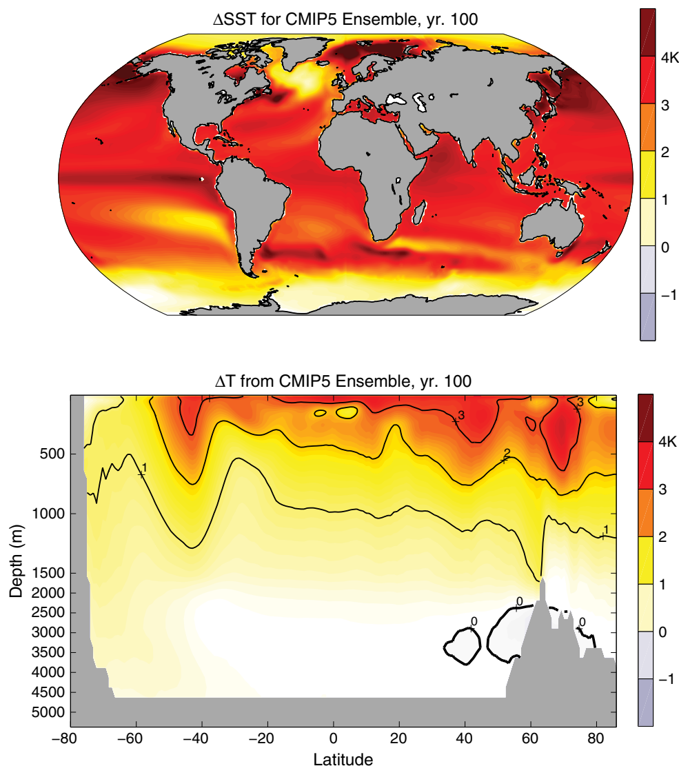
Fig. 1 Ensemble-average ocean temperature change after 100 years from 15 CMIP5 models under a quadrupling of CO 2 : ( top ) at the sea surface ( bottom ) in the zonal-average (contoured every degree K). Note the expanded scale in the top 1,500 m. The 15 CMIP5 mod-
