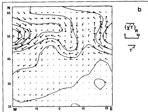
FIG. 2. (a) Scatter diagram of \delta\overline{T} (K) and \delta\overline{h} (in dam) at 400 mb, showing their functional relationship. (b) advection eddy heat flux (\overline{\mathbf{V}'T'})_R ( \text{ms}^{-1} \text{K} ), Eq. (4), plotted against \overline{T'^2} (C.I. = 3 \text{K}^2 ). The constant of proportionality d\overline{\psi}/d\overline{T} is calculated from the gradient of the straight line drawn through the points of Fig. (2a). This flux is non-divergent.
