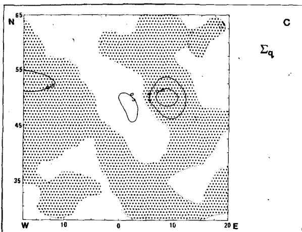
FIG. 8. The spatial distribution of the terms in Eq. (6) at 300 mb (C.I. = 3 \times 10^{-15} \text{ s}^{-3} ). (a) \bar{V} \cdot \nabla_h \bar{q}^2 / 2 , (b) (\bar{V}'q)_R \cdot \nabla_h \bar{q} and (c) their sum \Sigma q . Shaded regions are negative, unshaded regions positive.
