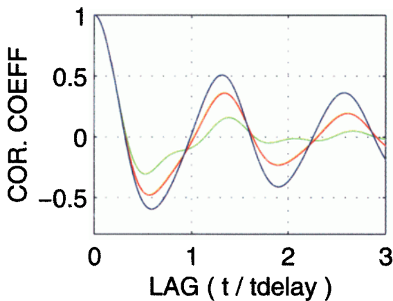
Plate 2. Low-pass autocorrelation function of the model NAO for various q -factors ( q = 2 , green; q = 5 , red; q = 10 , blue). Low-pass filtering has been constructed by only including periods greater than 5 yrs when computing the Fourier spectra.
