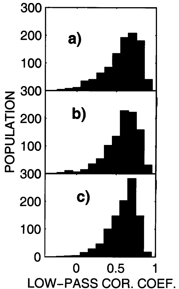
Figure 2. Histograms of low pass correlations between \tau^C and \tau^E obtained from 1000 simulations of (9), (10) and (11) (a) g = 0 (BB's model) and (b) q = 2 , (c) q = 10 (M99's model).
