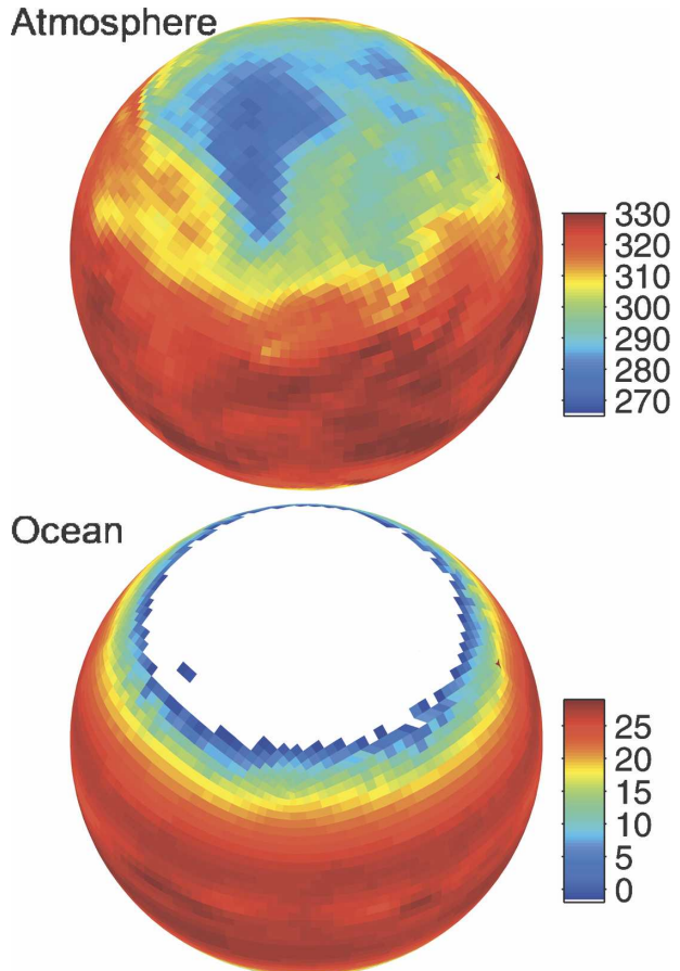
FIG. 1. (top) A snapshot of atmospheric temperature (K) at 500 mb revealing the presence of synoptic systems. (bottom) The SST ( ^\circ\text{C} ) and ice distribution. The underlying cubed sphere grid can be seen.
